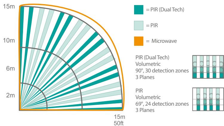
TMD15 Horizontal coverage
