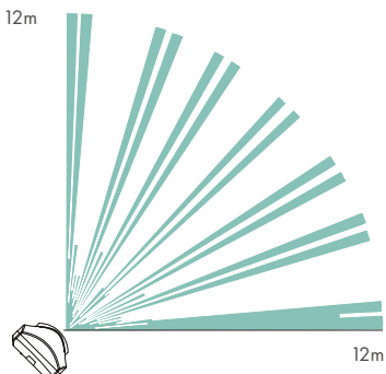
Horizontal coverage
