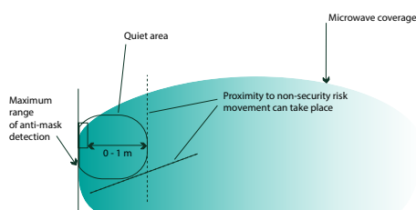
Anti-masking
