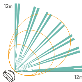
Horizontal coverage
