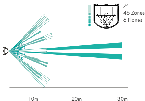
Horizontal coverage
