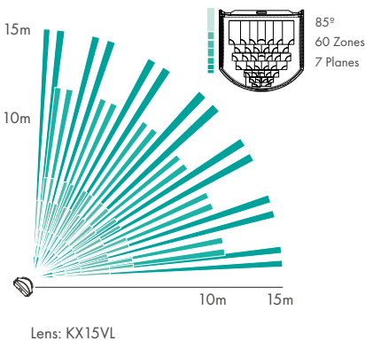
Horizontal coverage
