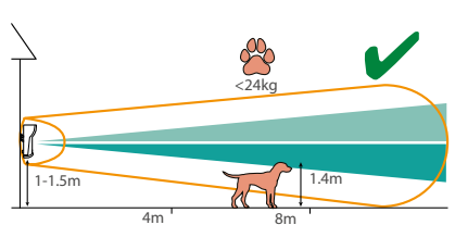
Vertical coverage
