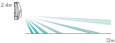
KX12DQ-WE - volumetric lens Vertical coverage
