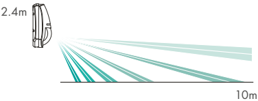
KX10DP-WE - volumetric lens Vertical coverage
