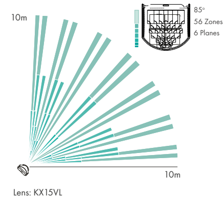
Horizontal coverage
