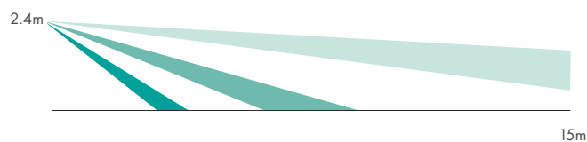
TMD15 Vertical coverage
